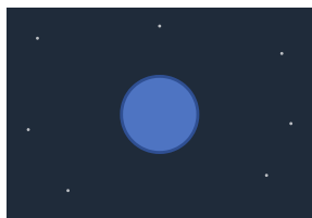
Neptune
