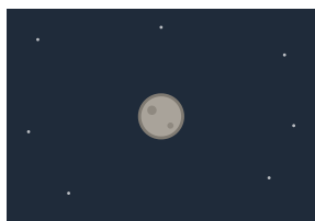
Mercure
